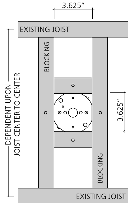
Fig. 3 - Blocking Detail
