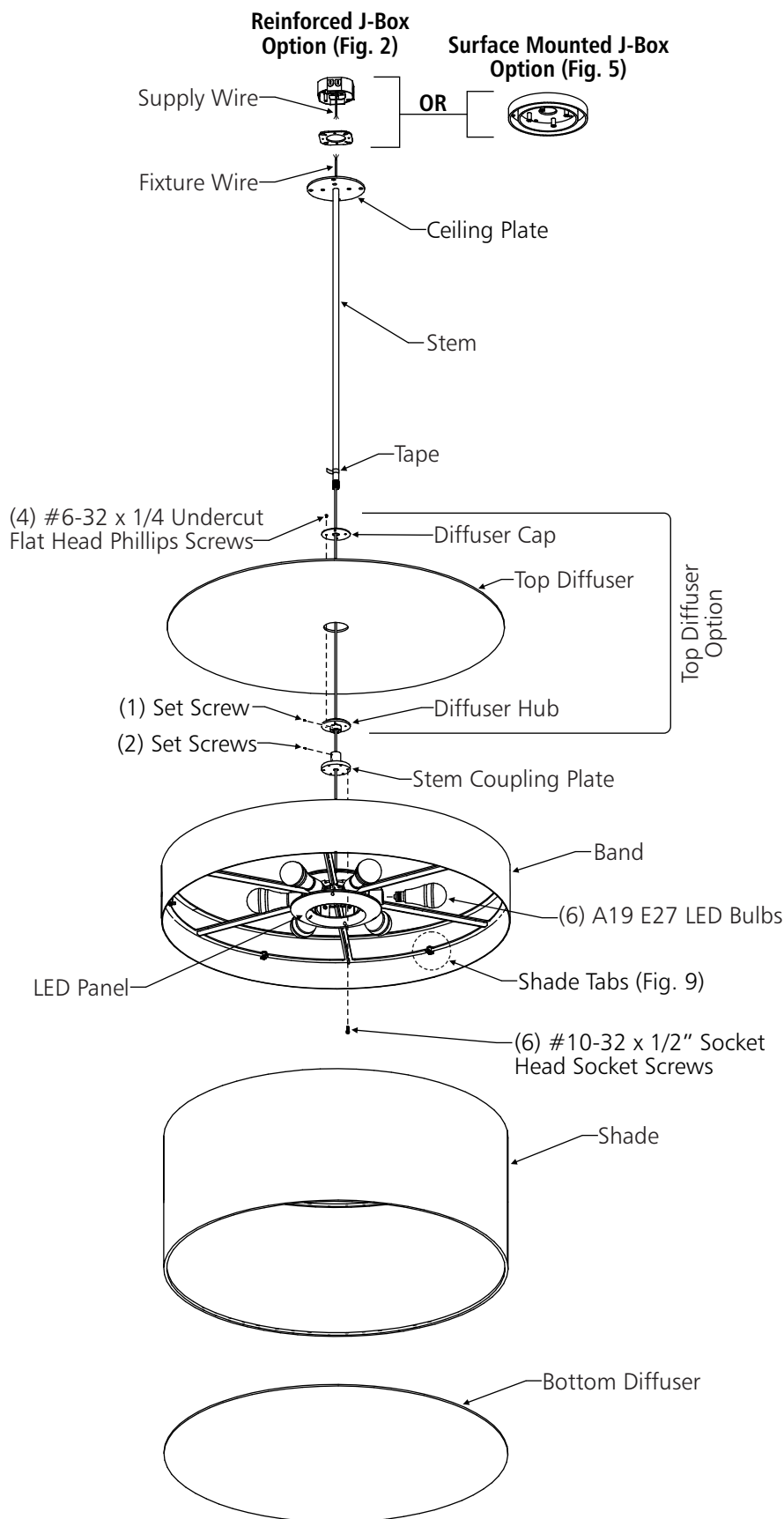
Fig.1 - Fixture Components
